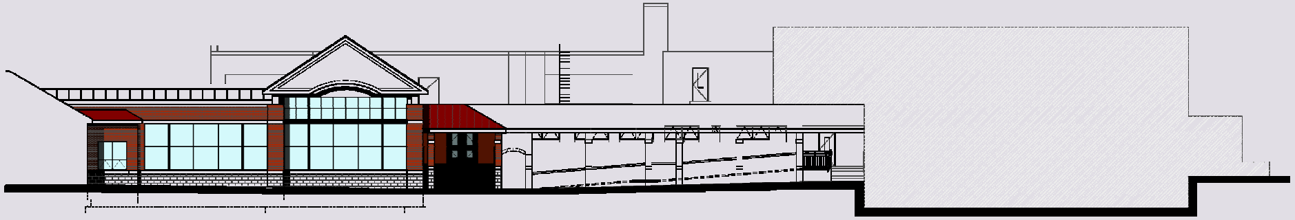
East Elevation
